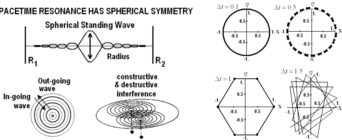
Figure 12. The Dirac polarized vacuum has hyperspherical symmetry. a) Top left, metaphor for TI standing-wave present showing future-past elements, R_1, R_2 , eleven of twelve dimensions suppressed for simplicity. b) Bottom left, top view of a) 2D spherical standing-wave; c) Bottom left right portion, manipulating the relative quantum/brane phase of oscillations creates nodes of destructive and constructive interference. d) Right, Four numerical simulations of the phase space trajectory of the Dubois superposed incurvise oscillator based on coordinates and velocities x_n = 1/2[x_n(1) + x_n(2)] v_n = 1/2[v_n(1) + v_n(2)] is shown in the figure for values of \Delta \tau = \omega t equal to 0.1, 0.5, 1.0 and 1.5. Initial conditions are \chi_0 = 1, \eta_0 = 0 & \tau_0 = 0 with total simulation time \tau = \omega t = 8\pi . Figure 12b adapted from [32].
