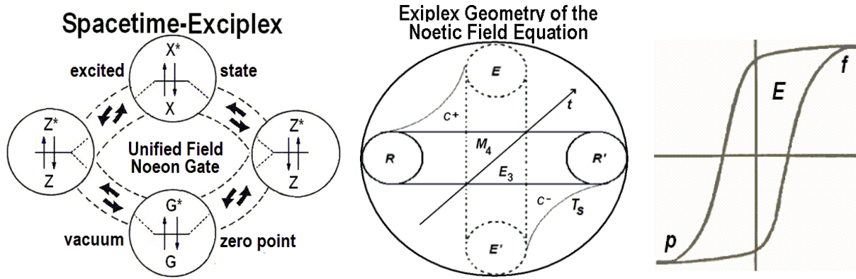
Figure 4. a) The geometry of the ‘spacetime exciplex’ (excited complex), a configuration of spacetime LCUs that act like a holophote laser pumping mechanism of U_F noeon energy and also how coherence of the U_F interacts with 3D compactified states in dendrons or microtubules for example. Locally the exciplex acts like an oscillating ‘cootie catcher’ [24]. b) Geometric representation of the Noetic Unified Field Equation, F_{(N)} = E/R for an array of cosmological LCUs. Solid lines represent extension, dotted lines field. Where F_{(N)} is the anthropic or coherent force of the U_F driving self-organization, total E equals the c) hysteresis loop energy of the hypervolume, R is the scale-invariant rotational radius of the action and the domain wall (curves) string tension, T_0 .
