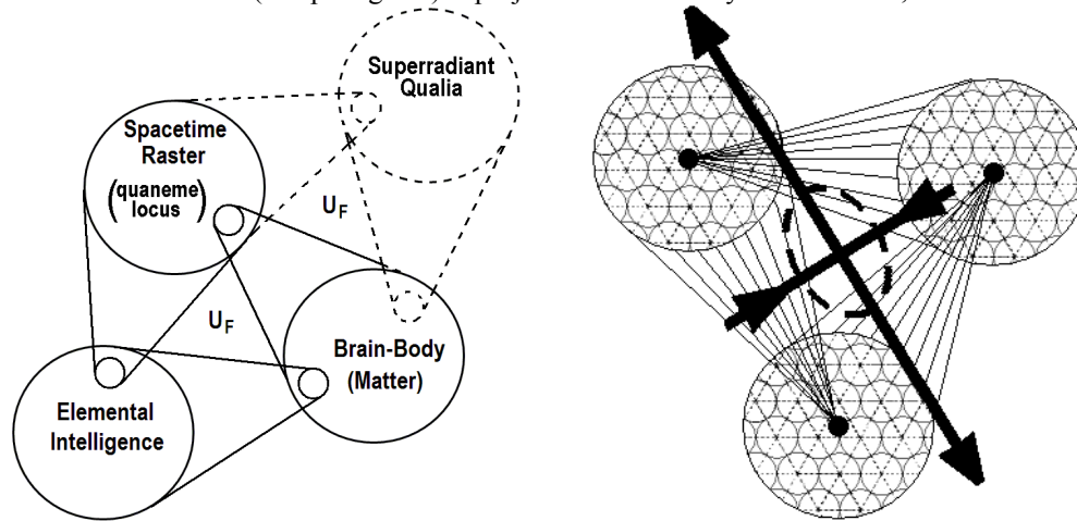
Figure 10. a) The physical basis of the continuous superradiant generation of qualia from the three components of mind: eternal Elemental Intelligence, Brain-Body (Descartes res extensa ), and the superradiant qualia (Descartes res cogitans ) mediated by the spacetime raster (quaneme locus) that exciplex gates 'the light of the mind' or U_F energy. The term quaneme is derived to parallel the phoneme component of sounds. b) LCU construct hidden nonlocally behind 3-space (black cross vertex).
