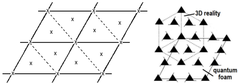
Figure 5. a) 2D view of the LCU tiling of the spacetime backcloth (Fig. 3). b) Projective geometry topologically giving rise to higher dimensionality (here the Fig. 4a) 2D view extended to 3D). The triangles with tails represent the trefoil knots in Fig. 6 and the naked triangles the resultant cyclic point or fermionic vertex quantum state in 3-space (Spheres in Fig.6).
