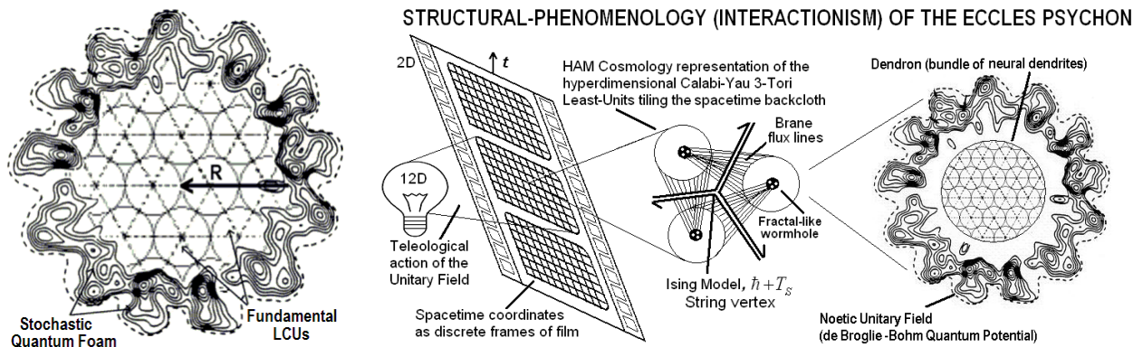
Figure 11. Conceptualization of Interactionist cosmology. a) Coherent interaction of the U_F bridging the stochastic quantum barrier into a brain dendron of radius R correlated with an underlying array of fundamental Least Cosmological Units (LCUs) forming the coupling of one Eccles Psychon unit with the brain. b) Showing injection of the noetic field or élan vital into spacetime points. c) Planck scale LCUs mediating the noetic field, d) An Eccles Psychon- U_F Noeon field coupled putatively to a brain dendron.
