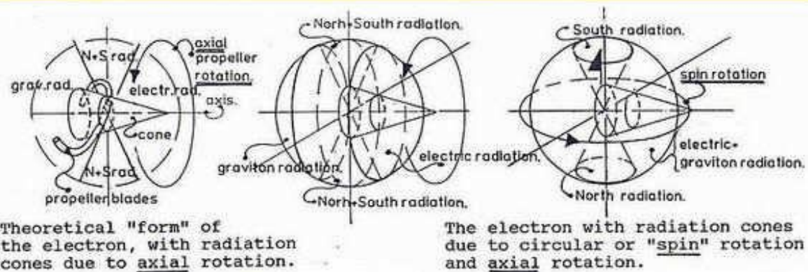
Figure 12, The polarisation of the double spinning propeller shape of Fermions is the origin of the monopole radiation differences radiated into different directions from the Fermion radiation area around the centre. It is assumed that electric and gravity radiation is not mixing with magnetic monopole radiation inside the magnetic double cone area. Consequently, the measured difference between the Equatorial gravity (9.78 m/sec 2 ) and Polar gravity (9.83 m/sec 2 ) should be greater without this effect.
