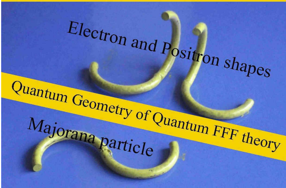
Figure 14, Three simple particle examples. The electron and Positron are each others mirror image. The Majorana particle has no mirror equivalent.
