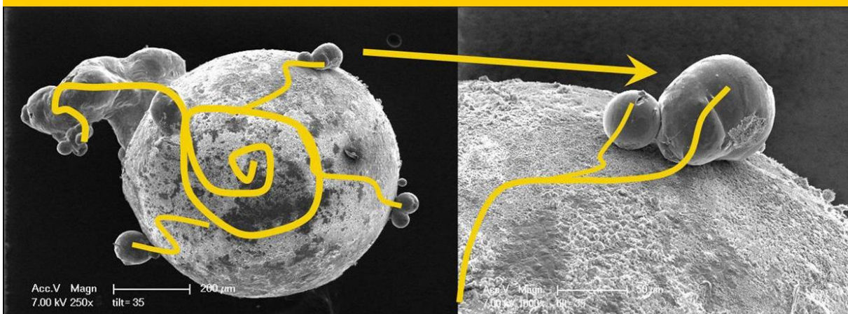
Figure 1. Comparison between LHC (CERN) UFO dust particles (10 \mu\text{m} ) with molten Silicon globules (100 \mu\text{m} ) originated in the lab by travelling and evaporating Interference Quantum Knots (micro dark Matter Black Holes)
