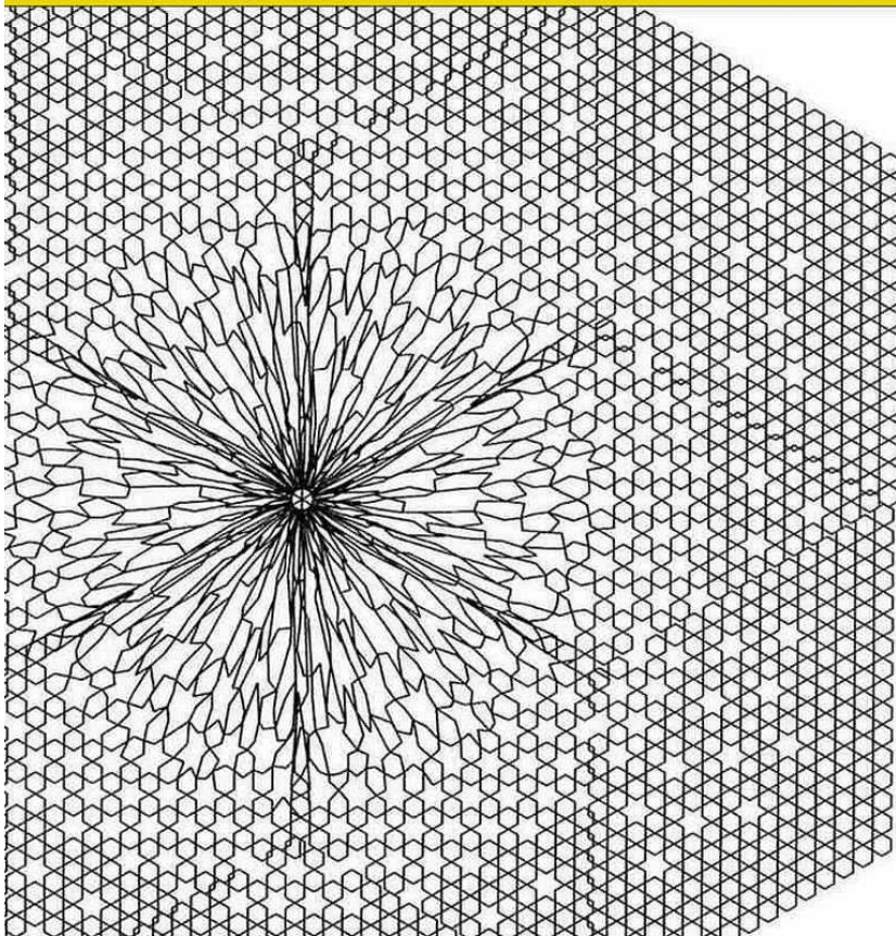
Figure 7, The Chirality and structure of the oscillating Dark Energy Higgs vacuum lattice
