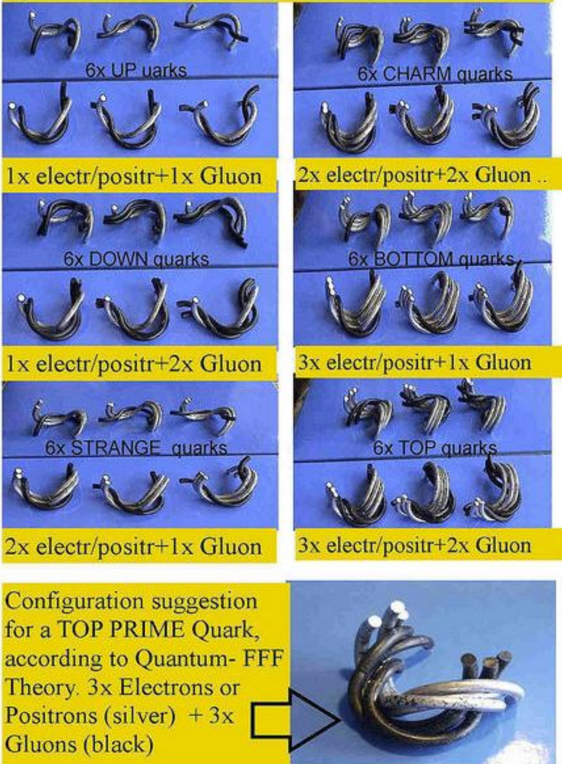
Figure 16, 5x different shaped Photon/Gluons can combine with the two propeller shapes of the Electron and Positron to form all coloured (QCD) Quarks and even a so called Top Prime Quark. The Muon and Tau particle are supposed to be the same as the Down quark, respectively the Charm quark.
