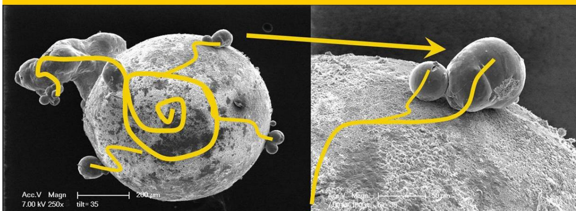
Figure 8, An other example of Quantum Knot heated globules found on an exploded battery. Suggestion for the origin of external stainless steel globules found on the Boeing 787 Dreamliner APU battery damage jan.7.2013 at Boston airport. Discharge Quantum Knot black holes seem to be able to melt stainless steel! Melting point of stainless steel is 3000 degree C! ( Globule diameter 30-120 \mu m.)
