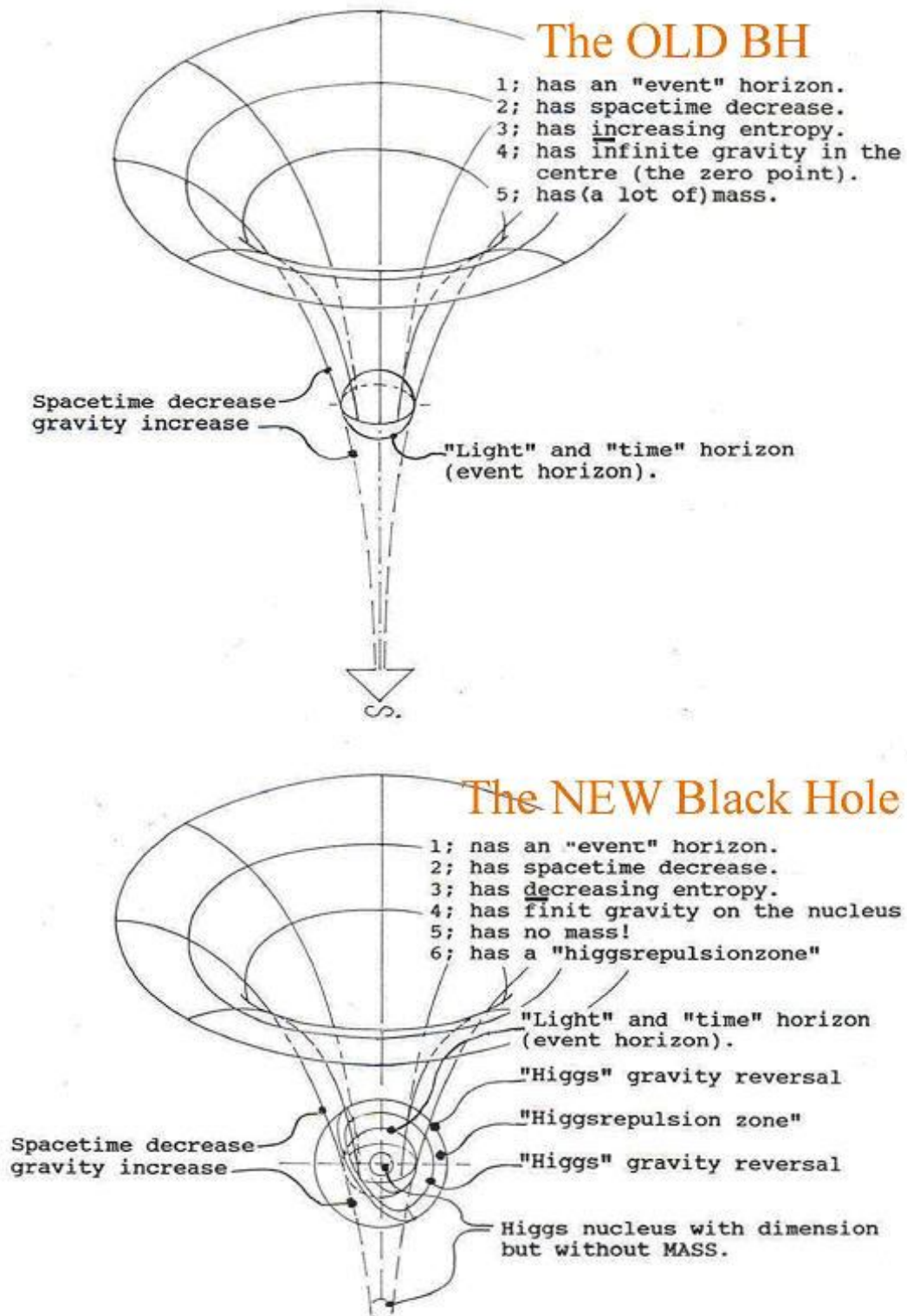
Figure 4, The difference between the old and new paradigm Black hole according to Quantum FFF Theory .
