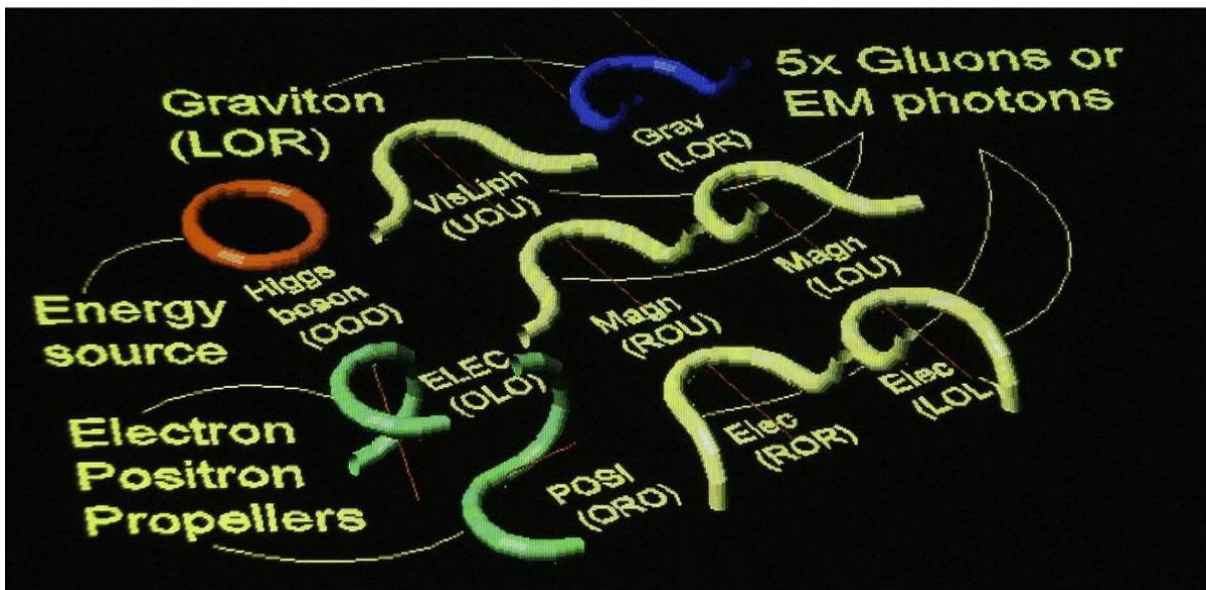
Figure 15, The particle zoo of single ELEMENTARY particles made out of ONE convertible Torus shaped Higgs particle, equipped with three hinges of 90 degree rotation.
