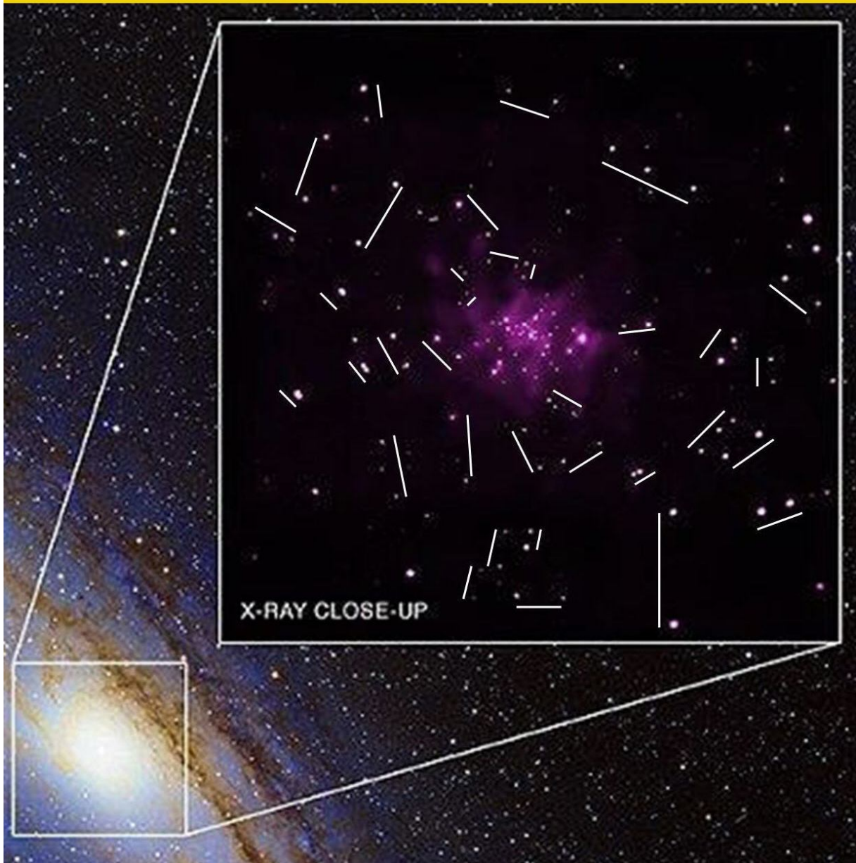
Figure 26, Pairing supernova black holes, as the origin of emergence of new open star clusters.
