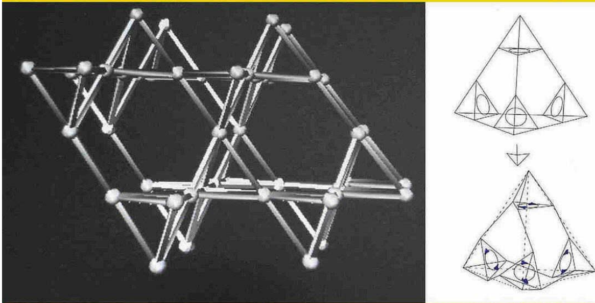
Symplified tetrahedral vacuum lattice structure (left), constructed by complex chiral tetrahedral building blocks (right). Each universe has to choose between a left- or righthanded rotation of its tetrahedral building blocks. Each chiral lattice has the Planck length and is supposed to be equipped with at least two oscillating massless new Higgs particles.
