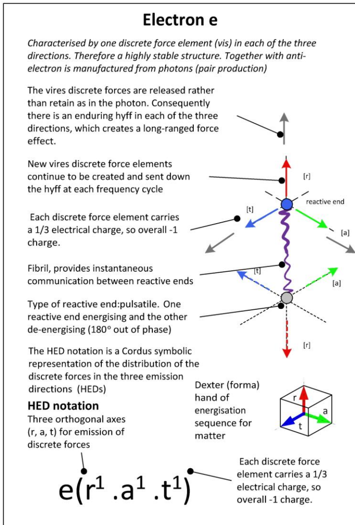
Figure 3: Cordus model of the electron. It is proposed that the particule has three orthogonal discrete forces, energised in turn at each reactive end.
