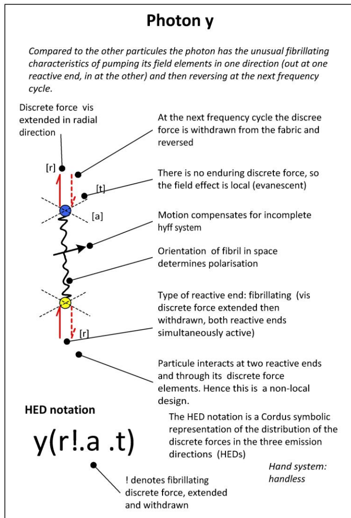
Figure 2: The Cordus model for the photon structures.
