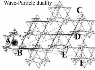
Photon trajectories through the tetrahedral Chiral vacuum lattice.
