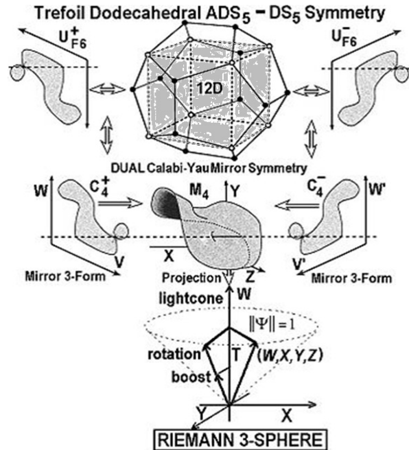
Figure 5. Complete LSXD regime of HAM cosmology illustrating the hierarchy of its geometric topology. Dodecahedral involute properties, as well as the continuous-state exciplex 'hysteresis loop' of neon injection not shown. It represents a unique M-Theoretic model of 'Continuous-State' U_F dynamics as it relates to NFT and its putative exchange quanta of the U_F called the neon.
