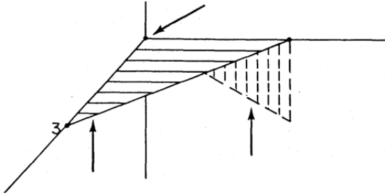
Figure 14. We illustrate an example in which a real space-like separation of events P_1 and P_2 appears to be contiguous by the introduction of the complex time, t_{xRe} + it_{xIm} such that from the point of view of event P_3 , the time-like separation between (x_2(P_2) - x_1(P_1)) appears to be zero.
