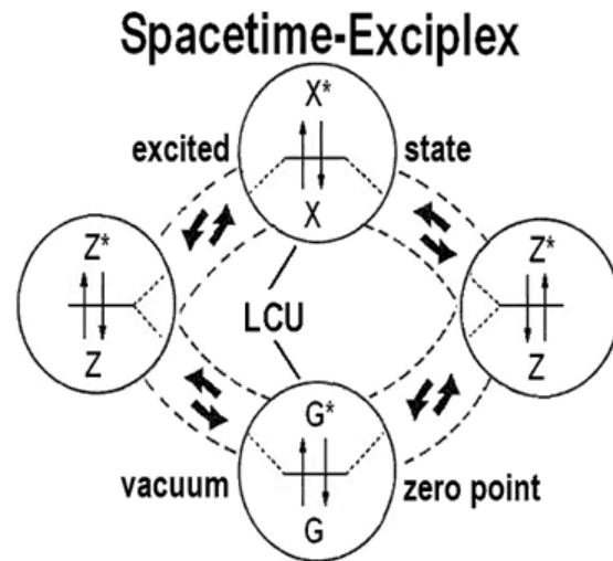
Figure 8. Least Unit (LCU) Exciplex Composite. The spacetime exciplex complex is comprised of an array of least cosmological units that act as a brane topology gating mechanism for entry of unified field control parameters to operate on Minkowski 4-space.
