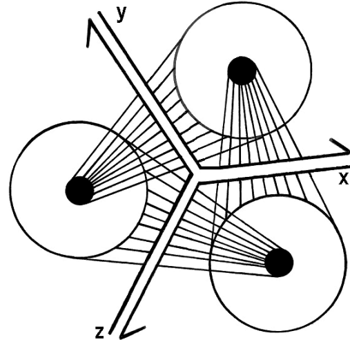
Figure 7. Triune structure of a solitary least unit that like an isolated quark does not exist in nature. The central parallel lines are the Witten string vertex with properties of a complex Riemann sphere able to continuously rotate from zero to infinity. The field lines represent the 'super quantum potential' of the unified field, U_F .
