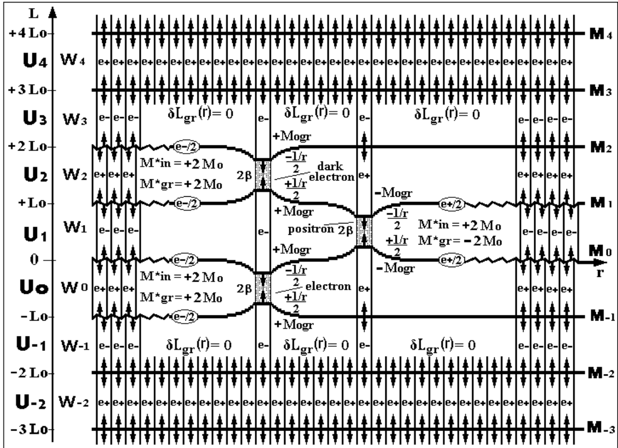
Fig. 4 shows schematically fragments of the L_{oe} -periodic 4D-space with endless number of quasiflat, adjusted and 3D-waveguides W_n , formed by the stretched quasiparallel 3D-membranes M_n ( n=0, \pm 1; \pm 2; \pm 3 \dots ). All waveguides are densely filled by intrinsically identical e -cells. Each even waveguide W_{2n} (by convention) contains monolayer of electron cells ( e -cell), and each odd waveguide W_{2n+1} contains adjacent monolayer of positron cells ( e -anticells), carrying the same dynamical energy E_4 = M_e C_4^2 > 0 and positive inertial mass M_e > 0 . Each e -cell is coupled with its adjacent e -anticell, realizing weightless (composite-made) superfluid vacuum, built from ( e^-/e^+ ) bosons. Adjacent monolayers W_{2n} and W_{2n+1} confine identical e -cells, which are strictly divided by the dividing joint membranes M_{2n} and cannot “annihilate” – but instead they are strongly - electrostatically pairwise coupled and build 2L_0 -periodic coupled monolayers/anti-monolayers of scalar ( e^-_{2n} / e^+_{2n+1} ) bosonic “atoms” – non-gravitating , chargeless and spinless multilayered “grains” of the 3D-vacuum-superfluid at low T. Periodic matter and antimatter particles arise in the layered PWM-vacuum strictly symmetrically as e -holes and e -antiholes and are shown in three waveguides:
