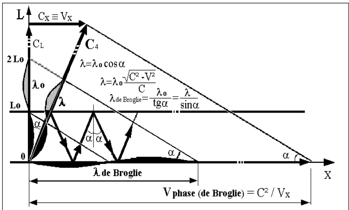
Fig. 1.1 shows three basic intersections of the C_4 -wave, propagating in the 3D-waveguide (x, y, z, 0 < L < L_0) . This wave propagates, being reflected along a polygonal trajectory \uparrow \downarrow \uparrow \downarrow \uparrow \downarrow \uparrow \downarrow C_4 t with the corresponding co-phase waveguided conditions (see Fig 1.2a), simultaneously creating pure C_4 -dynamical “frozen” - quantized “rest mass” harmonics ( OL -wave crosssection) with the waveguided-emergent SR, the wave of de Broglie ( OX -wave crosssection) and physically obvious Kaluza’s “cyclical conditions”.
