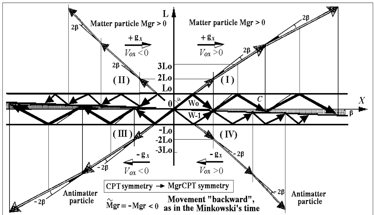
Fig. 2c shows the quasi-linear curved C_4 -sweep of the C_4 -sloping waveguide’s trajectory in the imaginary - periodically unrolled ( x,L ) corresponding one-layered waveguide’s spaces. We see (a) two matter particles (with initial particle velocity V_{0x} > 0 on the right side, and V_{0x} < 0 on the left side) in the above ( x,y,z,0 < L < L_0 ) matter-waveguide, which has positive opening ( \beta > 0 ), and correspondingly positive gravity acceleration g_x = dV/dt > 0 ; (b) two antimatter antiparticles are in the adjacent “antiwaveguide” ( x,y,z,-L_0 < L < 0 ) with the opposite – negative opening ( \beta < 0 ), and have negative gravity acceleration g_x = dV/dt < 0 (realizing by the same - middle dividing membrane non-parallelism \beta \approx 0 ).
