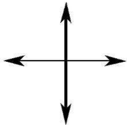
(Fig. 6, string theory might be applicable)
