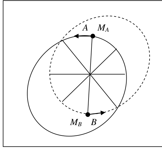
Figure 1: The orbit of the hypothetical binary star system \{A, B\} shown from above the orbital plane. The solid line represents the orbit of the primary (A) component and the dashed line the orbit of the secondary (B). The lines from the common center of mass towards the orbits indicate the relative positions of the periastron. The big dots indicate the relative positions of the stars at time of mid primary eclipse.
