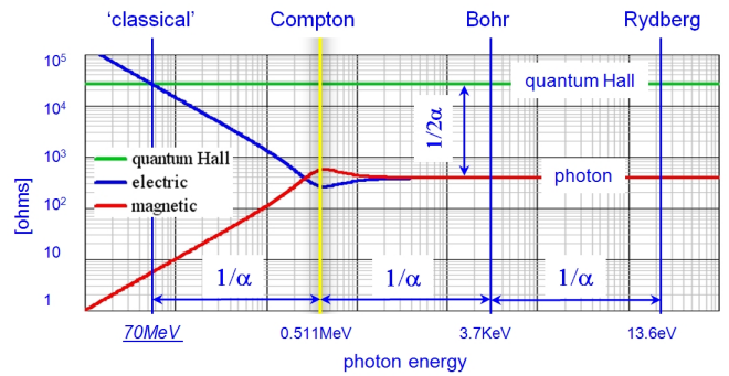
FIG. 1. Photon and electron impedances as a function of photon energy as defined by photon energy. The role of the fine structure constant \alpha is a prominent feature of the figure.
