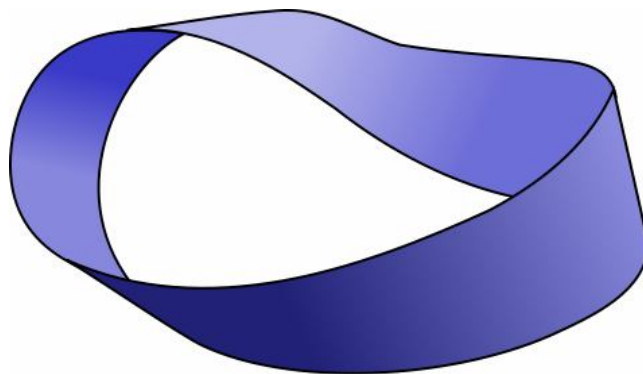
Mobius Strip
