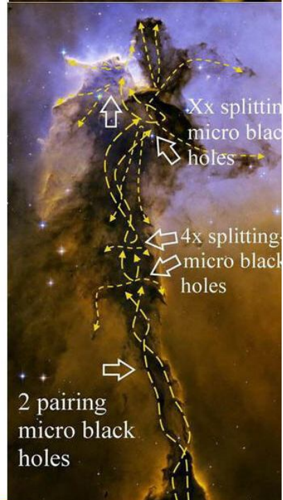
Figure 7. Pairing and Splitting Black Holes in Early galaxies Cygnus A and inside Nebula.
