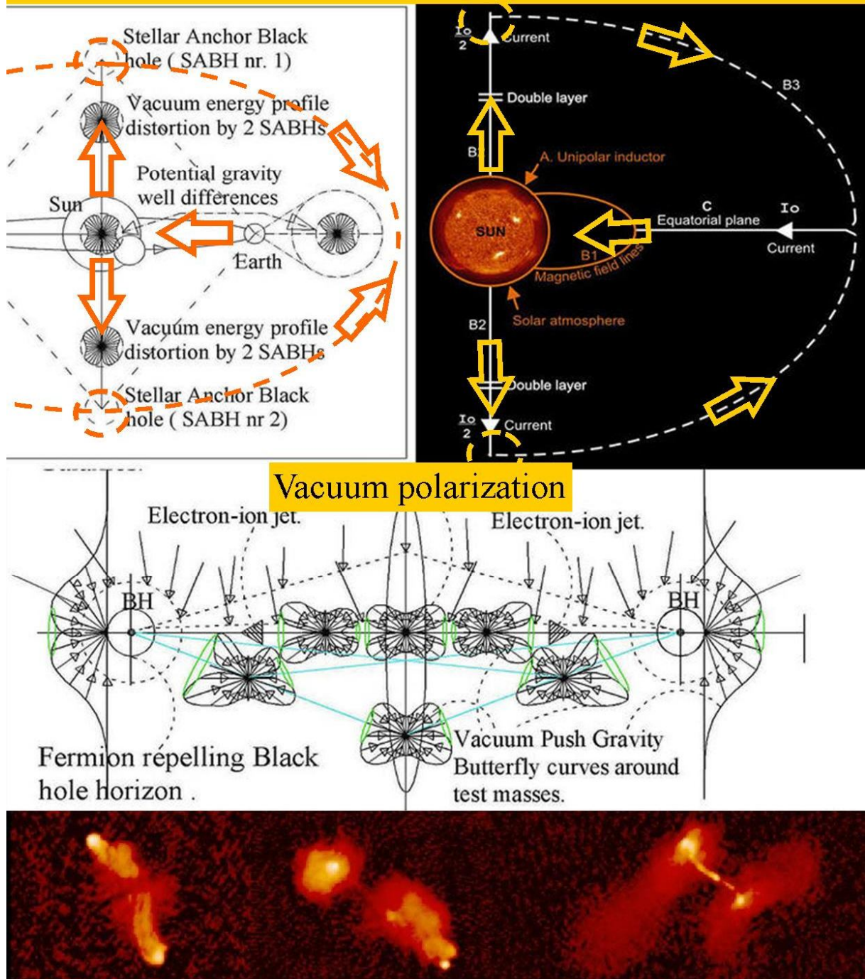
Figure 6. Oscillating Higgs vacuum polarisation with the resulting gas acceleration between black holes of difference sizes like Stellar Anchor Black Holes and Galaxy Anchor Black Holes.
