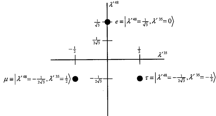
Figure 1: Three Generation Eigenstates Constructed from \lambda^{48} and \lambda^{35}
