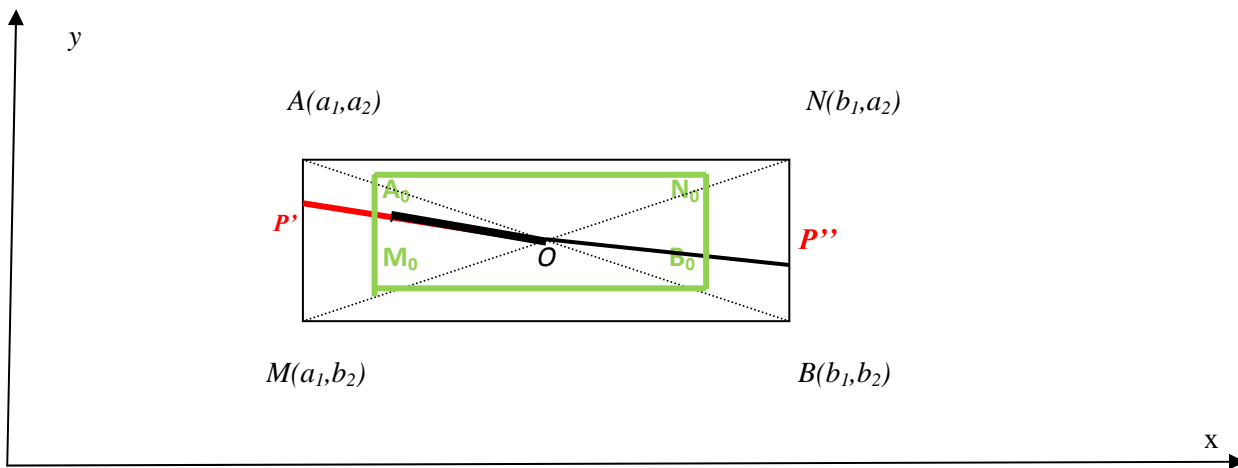
Fig. 9. The small rectangle shrinks until it vanishes.
