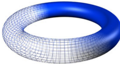
Figure 11. A Torus
