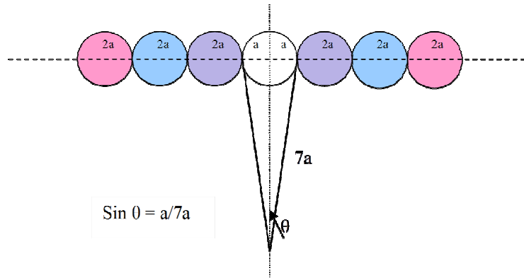
Figure 14. 3 Concentric Tori.
