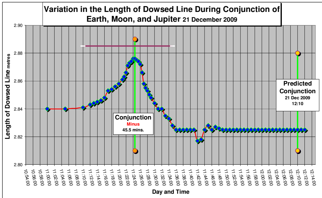
Figure 5 Measuring the Speed of Light from Jupiter
