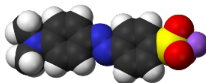
Figure 6: The 3D Structure of Methyl Orange
