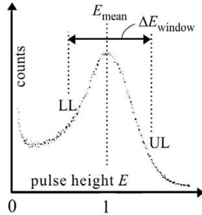
Fig. 1 PMT pulse-height response.
