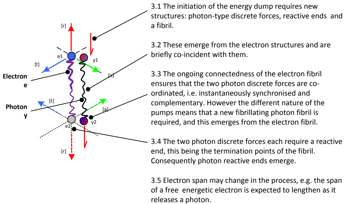
Figure 6: Prototype photon forms
