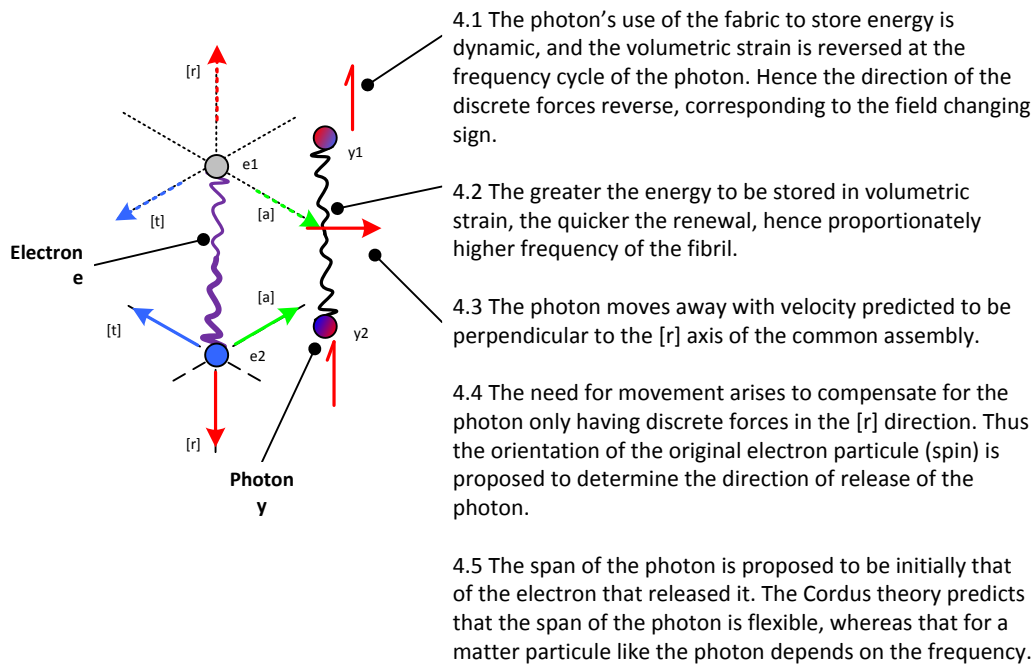
Figure 7: Photon separates from electron and moves off into fabric
