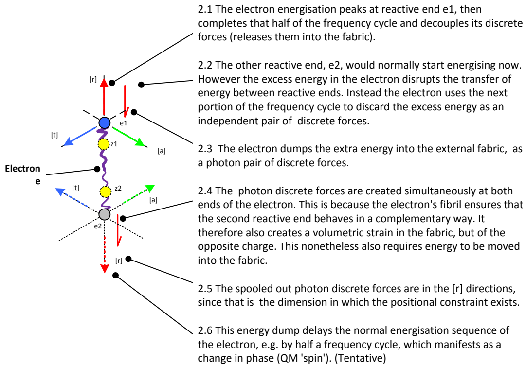
Figure 5: Electron dumps energy
