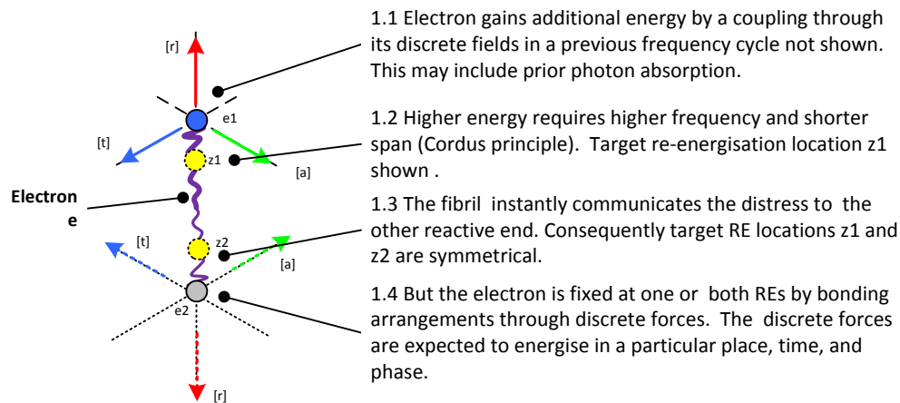
Figure 4: Energetic electron
