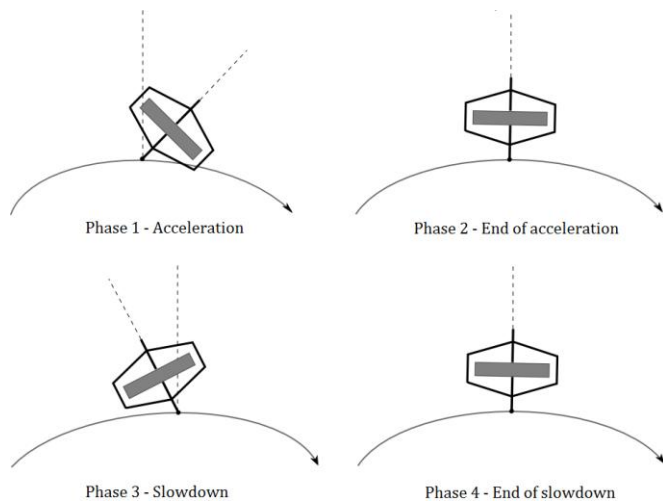
Fig. 11. Phases of gyroscope orientation relative to trajectory
