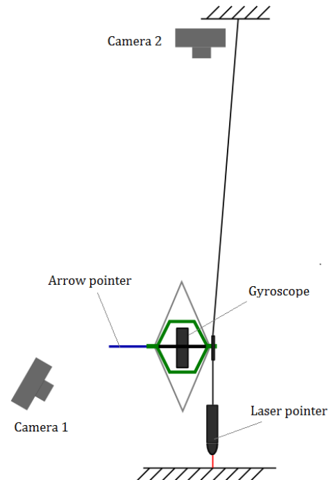
Fig. 1. Principle experiment setup
