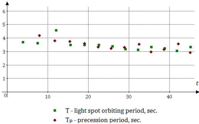
Fig. 9. Dependency of the light spot orbiting period and the gyroscope precession period on time
