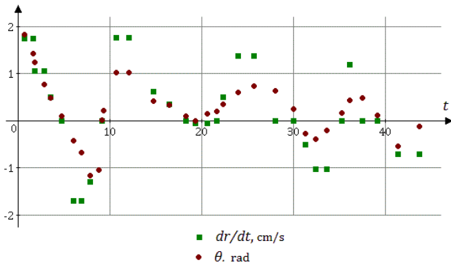
Fig. 8. Dependency of rate of change of polar radius, and the angle between spin axis and the normal line to the trajectory on time
