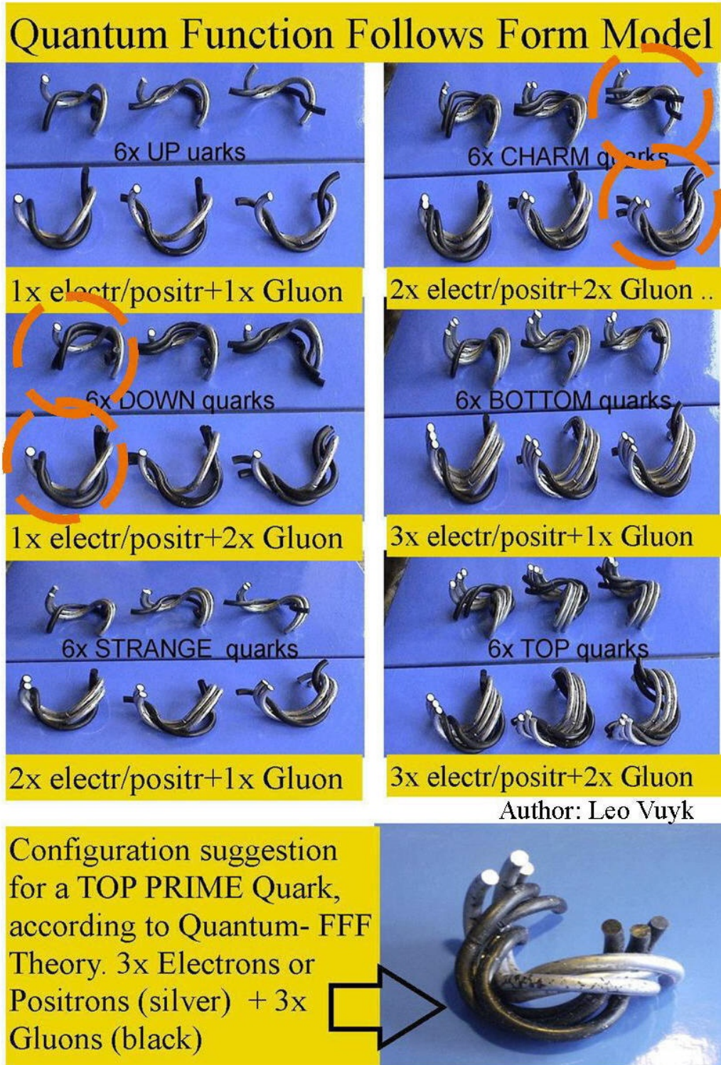
Figure 11, (in orange encircling: the assumed Muon (naked down quarks) and Tauon particles (naked Charm quarks))
