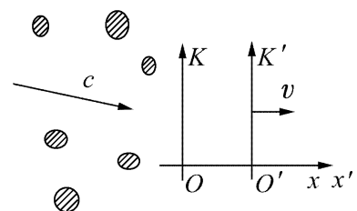
Fig 3.1 Is the light dependent on the frame of reference?
