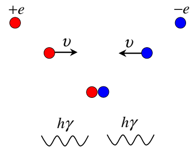
Fig 5.5 The sketch map of annihilation of electron and positron
