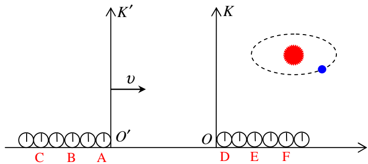
Fig 5.4 The observation of the same event from different frames varying widely
