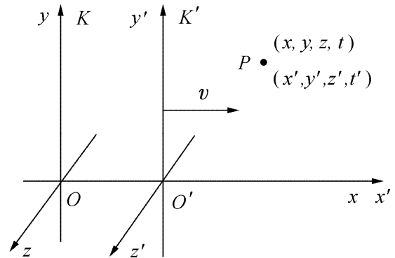
Fig 1.1 The sketch map of Lorentz Transformation
