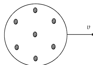
Fig. 5.3 the configuration of \mu^- meson
