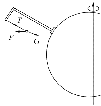
Fig. 5.1 Eötvös Experiment
