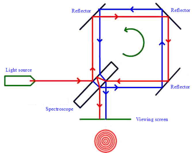
Fig. 3.5 Sagnac Effect
