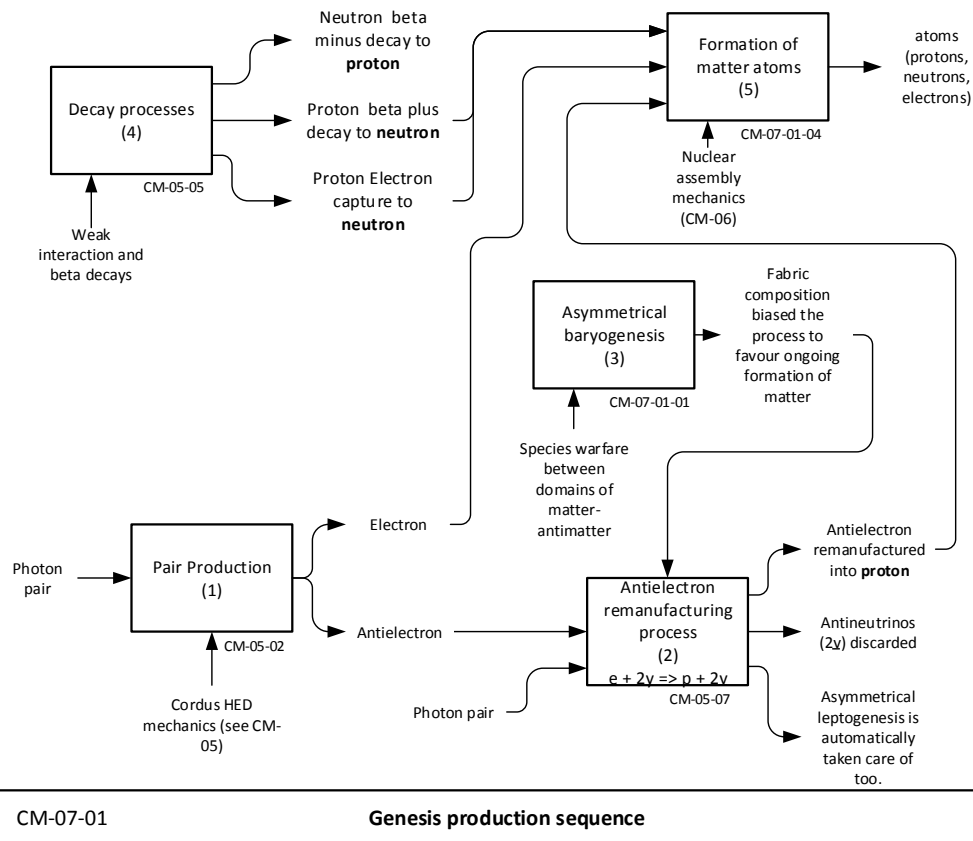
Figure 4: Genesis production sequence. Representation of the overall Cordus theory for the genesis production processes that resulted in matter.
