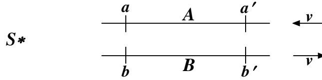
Fig.1 Test of Light Speed Invariance
