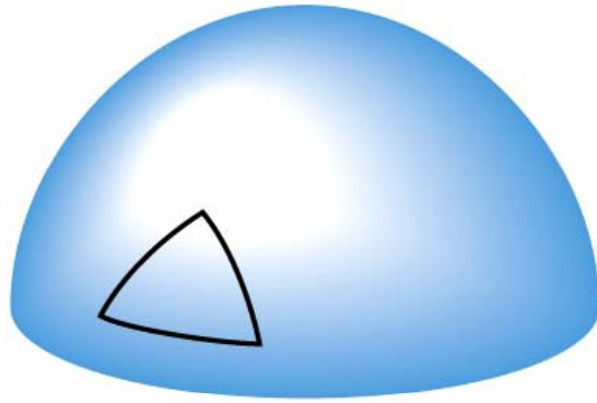
a Spherical space
