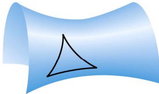
c Hyperbolic space
