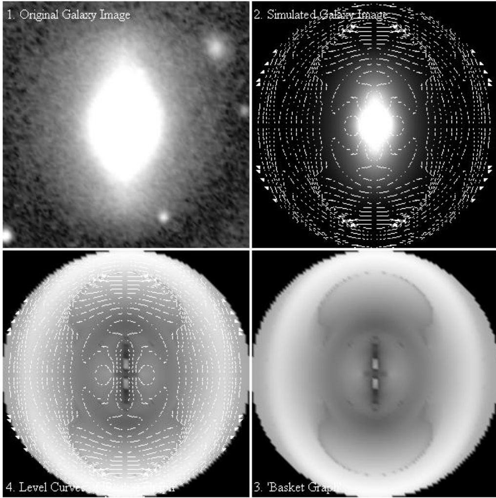
Figure 3: Upper left is a longer-wavelength image of barred spiral galaxy NGC 5701 (see [6] for image credit). Upper right is its simulation with an exponential disk and two dual-handle structures. Lower right is its ‘basket graph’ which is a demonstration of the function u(x, y) with the image brightness at each point being proportional to the corresponding value of the function. The function is the variance rate of f(x, y) along the direction of \alpha that is solved from instinct equation. Lower left is the level curves of u(x, y) which are simultaneously the proportion curves of barred galaxy. The curves are spider-shaped.
