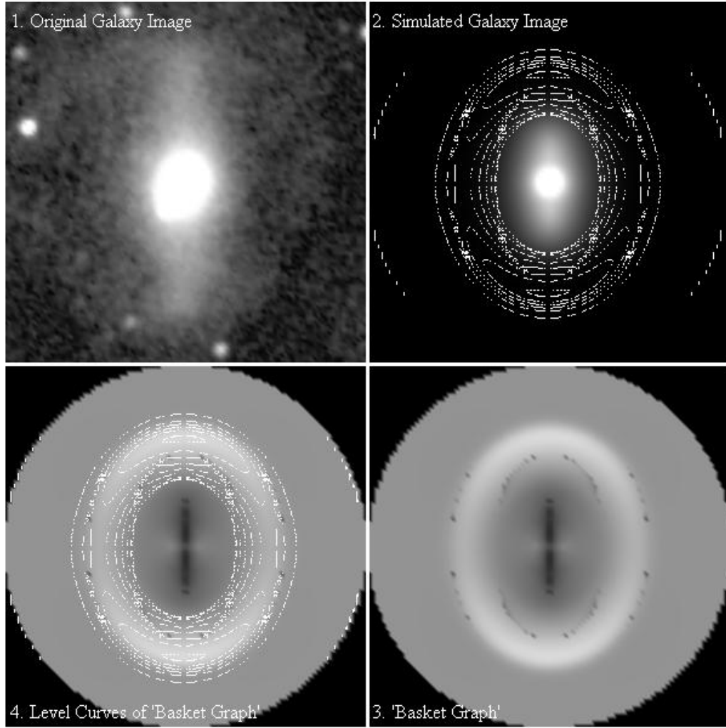
Figure 3: Upper left is a longer-wavelength image of barred spiral galaxy NGC 4930 (see [6] for image credit). Upper right is its simulation with an exponential disk and two dual-handle structures. Lower right is its ‘basket graph’ which is a demonstration of the function u(x, y) with the image brightness at each point being proportional to the corresponding value of the function. The function is the variance rate of f(x, y) along the direction of \alpha that is solved from instinct equation. Lower left is the level curves of u(x, y) which are simultaneously the proportion curves of barred galaxy. The curves are spider-shaped.
