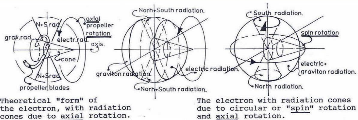
Figure 9, The Double spin of fermions, the radiation cones of different shaped monopole electro magnetic Photons and gravitons and the polarization effect on accelerated Fermions in a synchrotron device.
