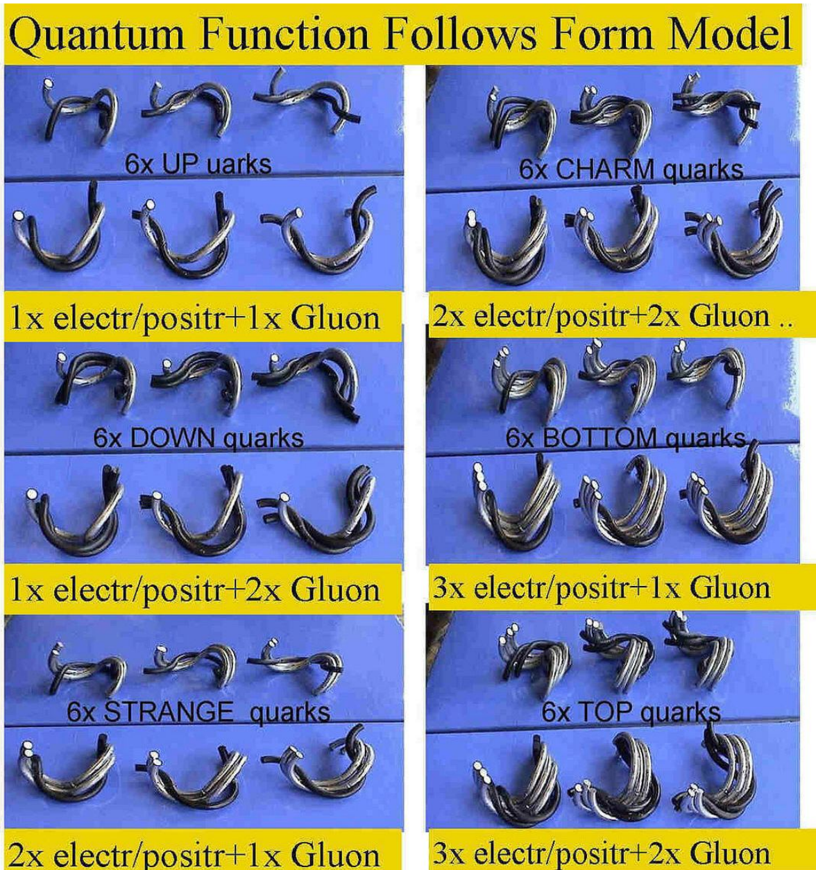
Figure 6, Alternative Standard Model for Quarks as composite particles of positrons, electrons and 5x gluons, able to create the different colors of Quantum Chromo Dynamics.
