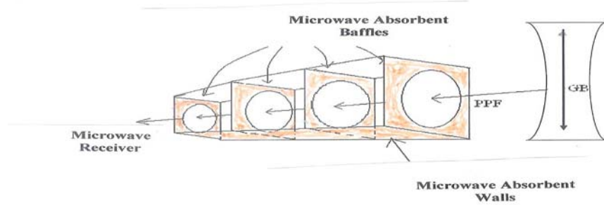
Figure 9. Schematic of microwave receiver shielded by MM absorbers and pyramid absorber/reflectors.
