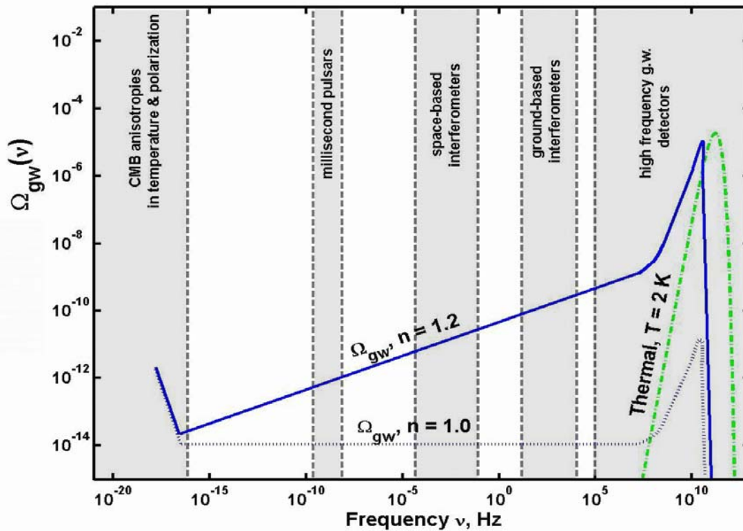
Figure 1. Predicted relic gravitational wave energy density as a function of frequency (slide 6, [42]).
