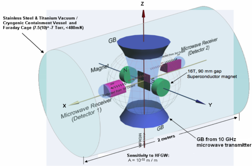
Figure 4. Schematic of the Li-Baker HFGW detector
