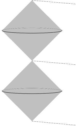
Figure 7: Pictorial representation of the double covering conformal infinity. Double double light cone. Points connected by a dashed line are, in fact, a one point. This representation is also topologically correct but differentially misleading.
