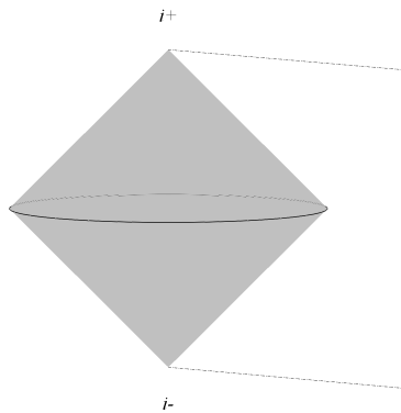
Figure 3: Pictorial representation of the conformal infinity with one dimension skipped. Double light cone at infinity with endpoints identified. While topologically correct this representation is misleading as it suggests non differentiability at the base, where the two half-cones meet.
