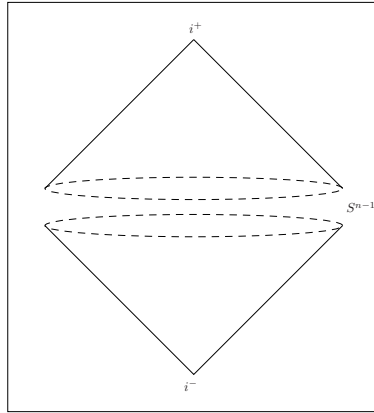
Figure 5: Chronological boundary for \mathbb{L}^{n+1} - Figure. 2 from [5]
