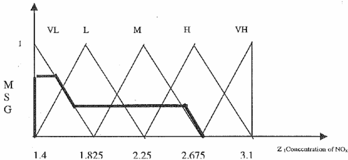
Figure 5.11: Aggregated output and defuzzification for the concentration of NO_x
