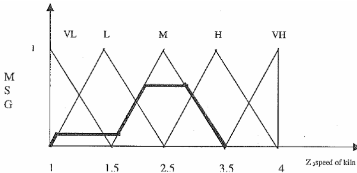
Figure 5.29: Aggregated output and defuzzification for the speed of kiln
