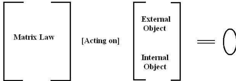
Figure 2.2 Prespacetime Equation
