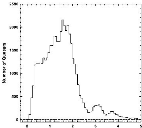
Fig. 1.1 : Distribution of 46,400 quasars with redshifts below z < 5 (Schneider et al. 2005).
