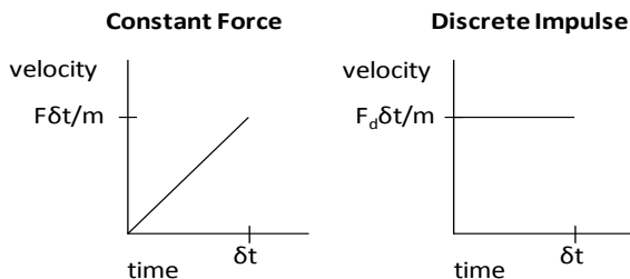
Figure 4: Shows the difference between a continuous constant force and a discrete impulse force. If the distances displaced are equal, the discrete force only need be half as strong.
