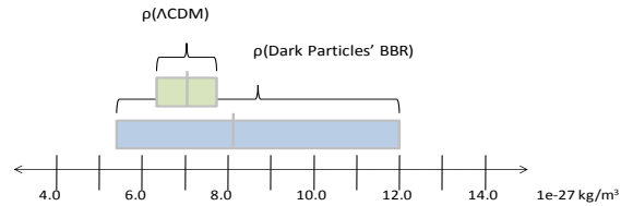
Figure 3: Visualization of density of dark energy from two models
