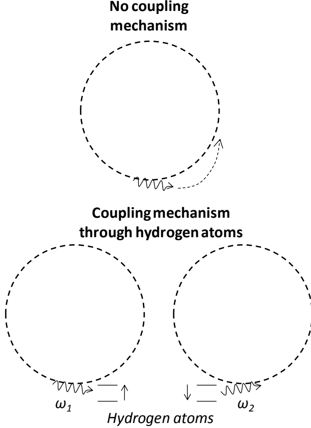
Figure 2: Without a coupling mechanism, the radiation can't obtain an escape trajectory thereby not allowing the dark particle to cool. However with a hydrogen atom or other sink the dark particle can equilibrate with the background radiation field.
