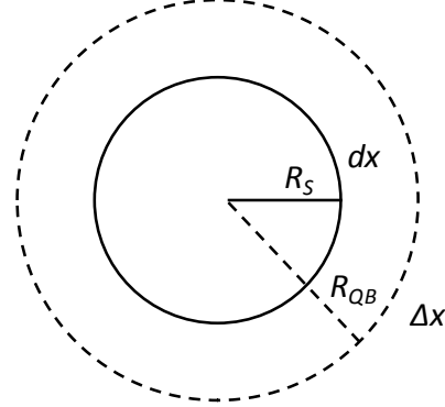
Figure 1: Event horizon and quantum boundary of black hole
