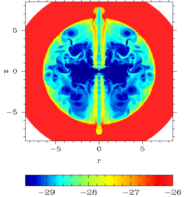
Figure 1. The plot shows \log_{10}\rho in dimensionless units. The unit of length in this and other plots is one light year.
