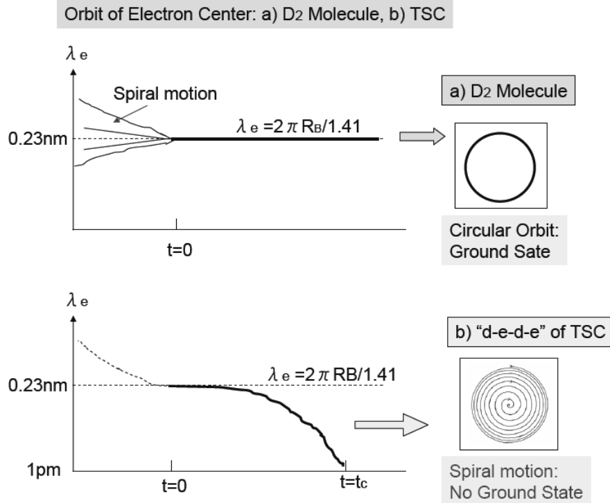
Figure 3. Time dependent behavior of effective electron wave length, a) D_2 molecule, b) “d-e-d-e” EQPET molecule of 4D/TSC
