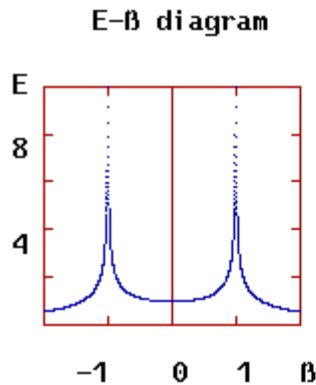
Figure 2.2. E-β diagram
