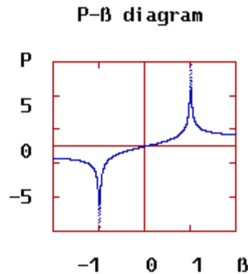
Figure 2.3. p-β diagram
